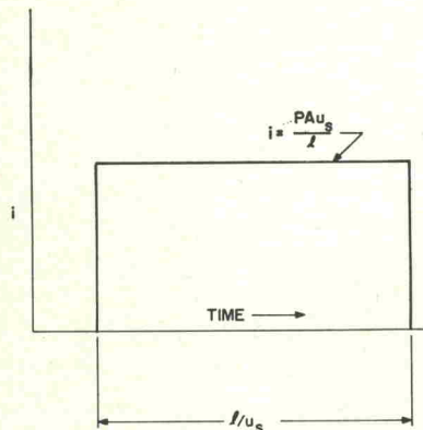
FIG. 2. Expected one-dimensional current waveform.
